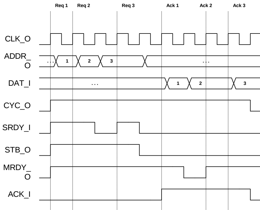
3-burst reads interrupted by slave and master
