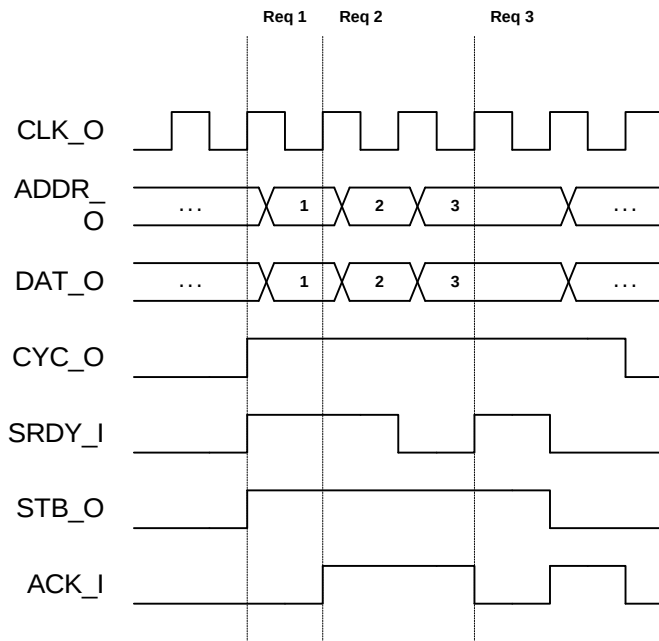
3-burst writes interrupted by slave
